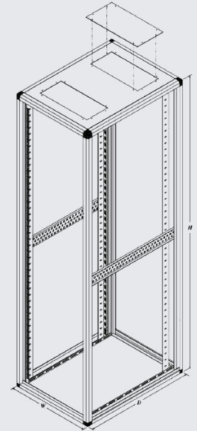
Standard Open Frame (Standard Cabinet Frame Parts)
